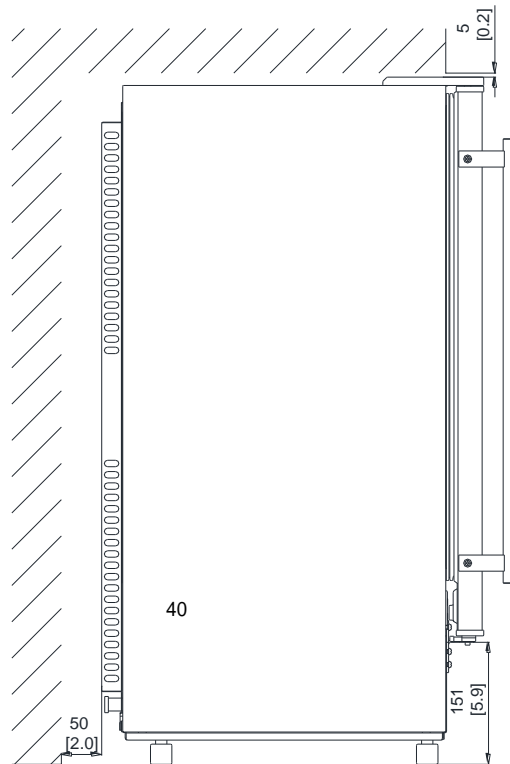
Side View (mm)
